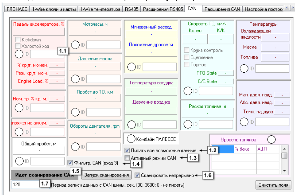
Рис.32 – CAN.
